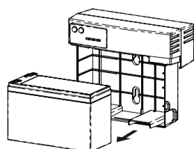
Step 2: a. Disconnect battery cable connector to remove battery. b. Replace with new battery and re-connect the battery connector.
